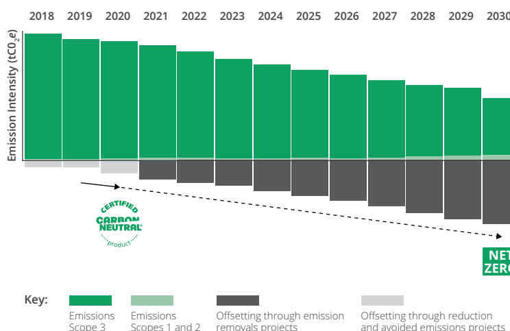
Figure 10: How CarbonNeutral® Certifications Support Net Zero Ambitions: Using CarbonNeutral® Product Certification to Start Taking Climate Action on Entire Value Chain Emissions
